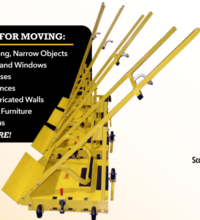
Upright position for loading, featuring several tilt settings for moving items (displayed with optional add-ons)
