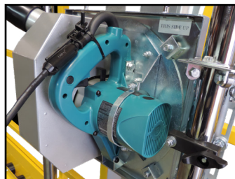
10" Saw on Spinning Insert + Dust Collection
