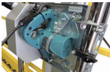
10" Saw on a Spinning Insert w/Dust Collection
